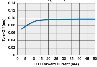
CPC1988 Typical Turn-Off vs. LED Forward Current ( I_L=0.5A )
