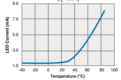
CPC1988 Typical I_F for Switch Operation vs. Temperature ( I_L=0.5A )
