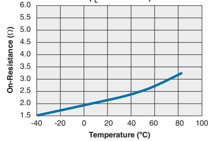
CPC1988 Typical On-Resistance vs. Temperature ( I_L=\text{max rated} )
